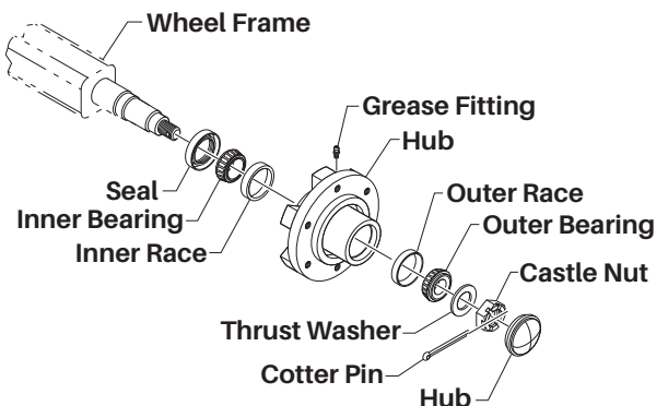
Figure 2-2. Wheel Hub
