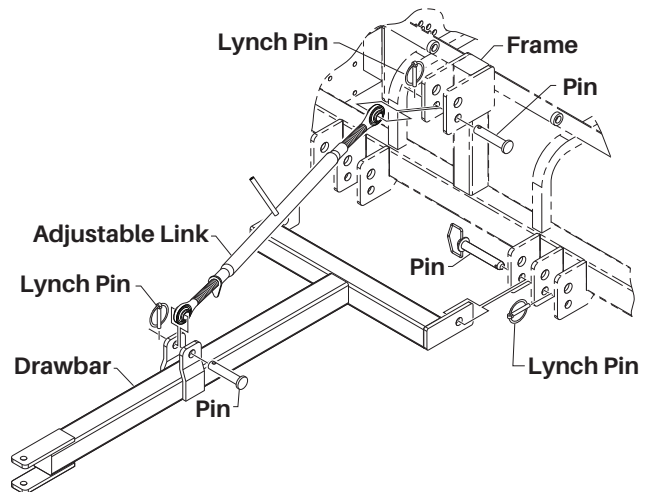
Figure 1-2. Drawbar attachment
