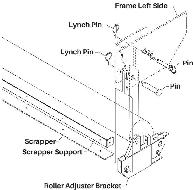
Figure 1-4. Roller adjustment
