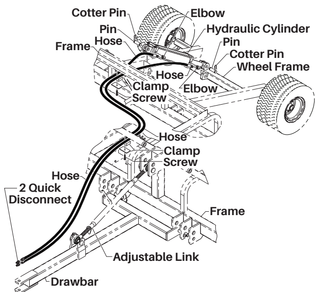
Figure 1-3. Gauge wheel attachment
