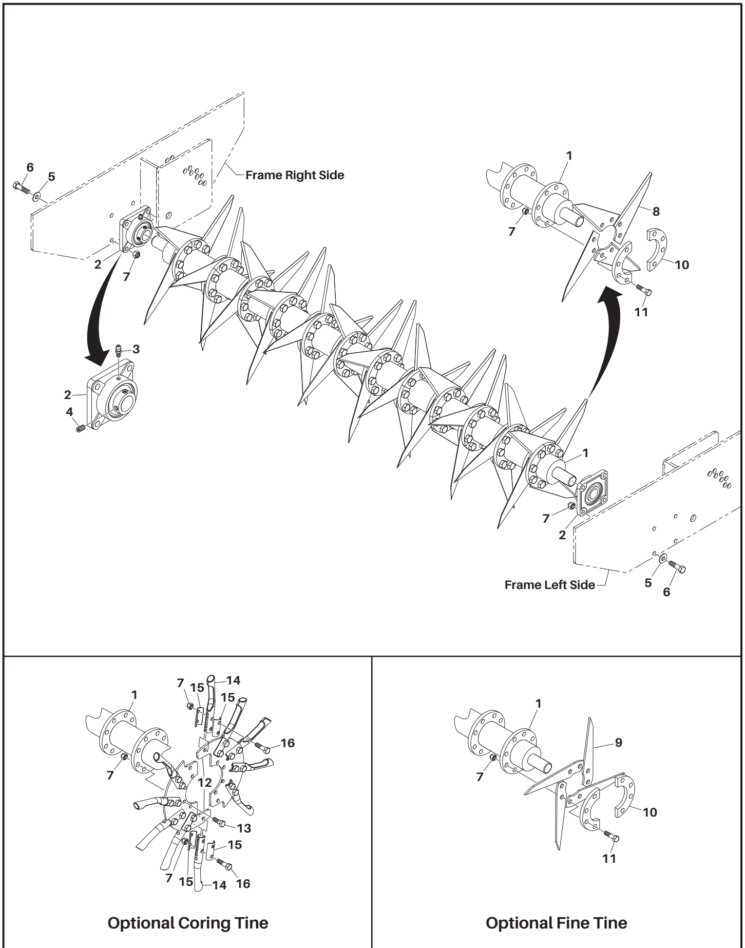
Figure 3-2. Rotor, Tines and Related Parts
