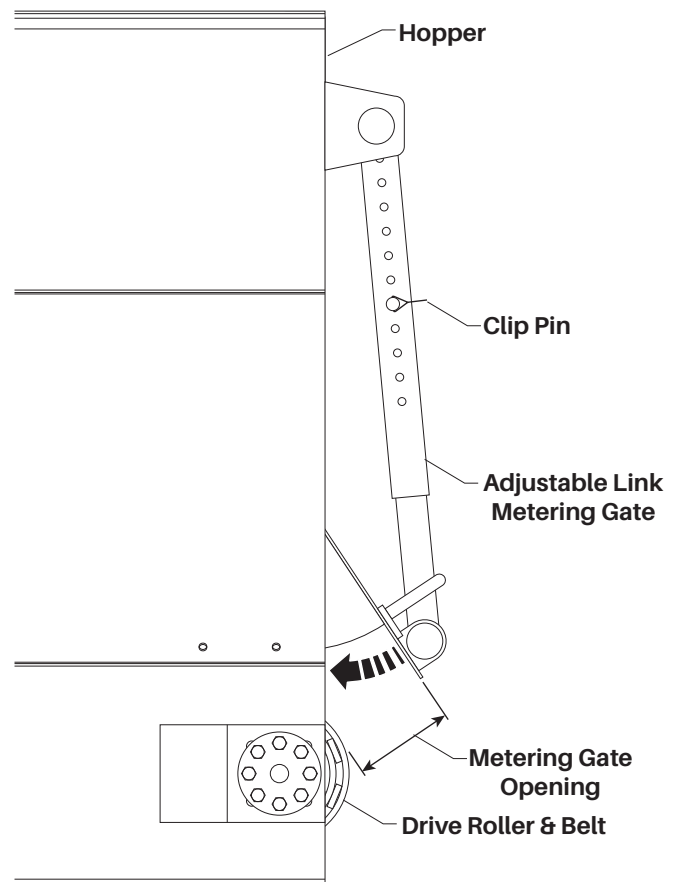
Figure 1-1. Metering Gate Adjustment
