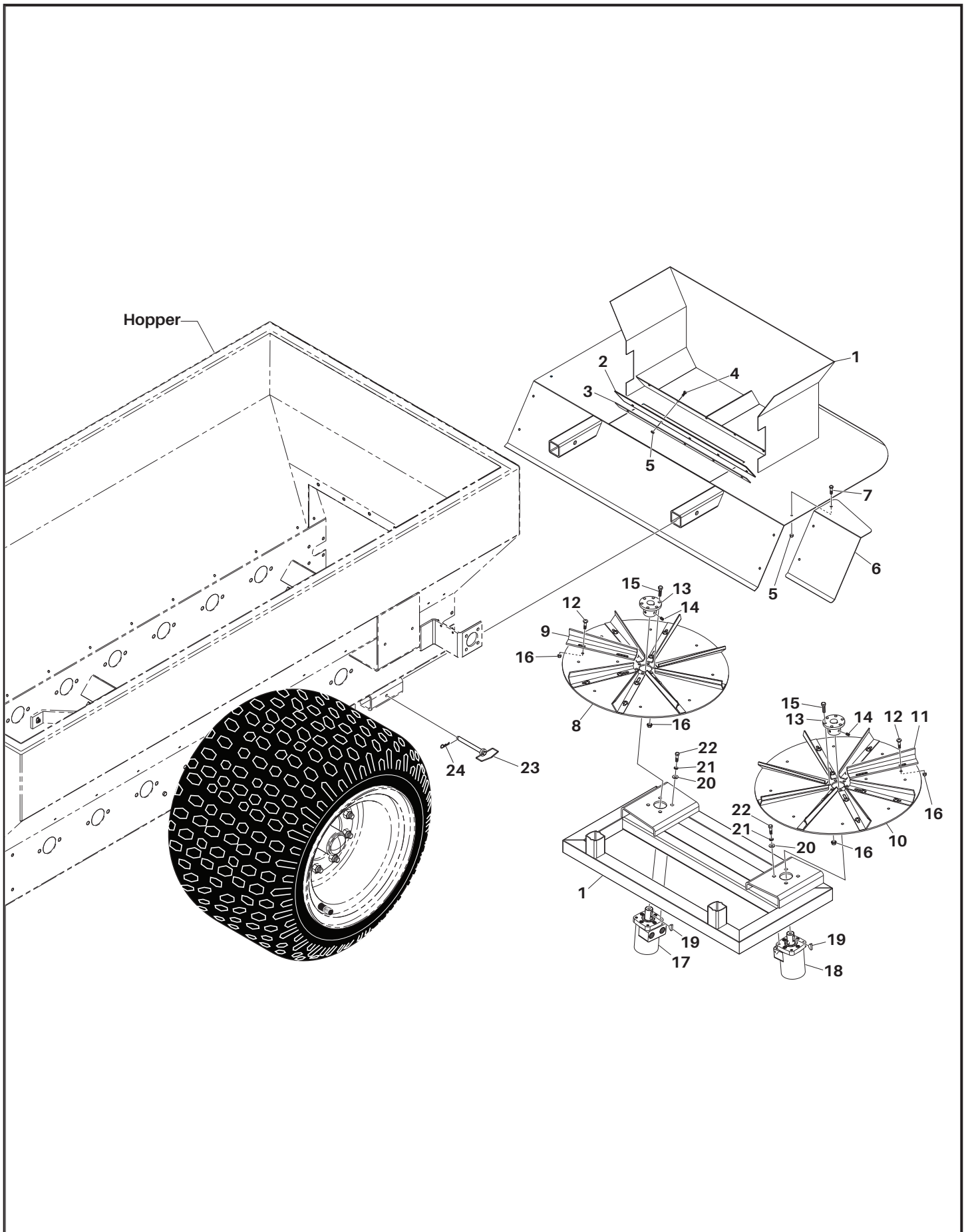
Figure 3-4. Spinner Attachment and Related Parts
